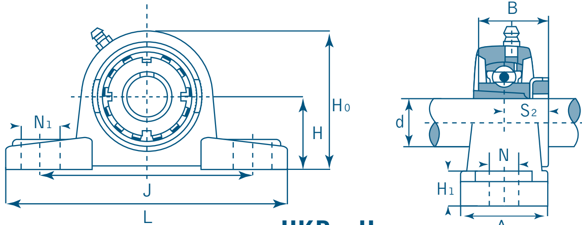
UKP + H Adapter Sleeve Locking
