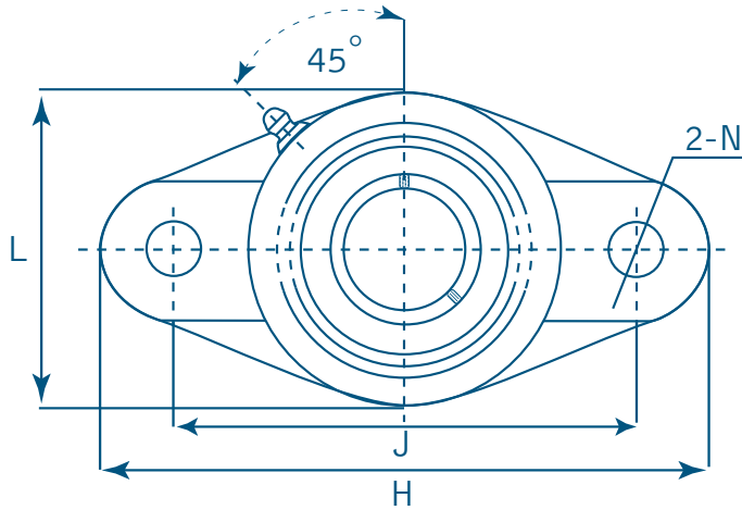
UCFT Set Screw Locking
