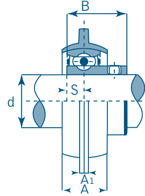
SBPFL Set Screw Locking
