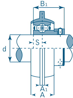
SAPFL Eccentric Locking Collar
